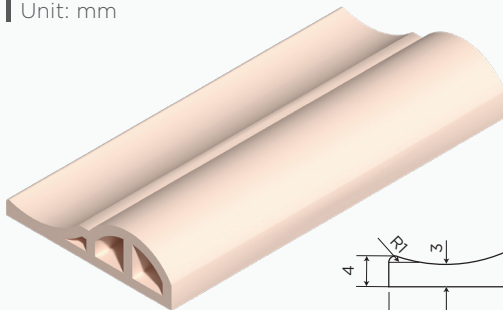
Hollow Moulding Unit: mm
